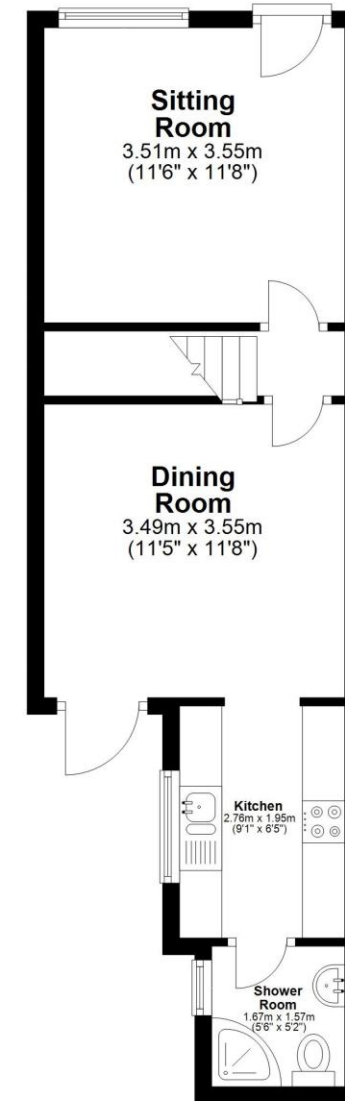
Ground Floor Approx. 36.6 sq. metres (394.5 sq. feet)
